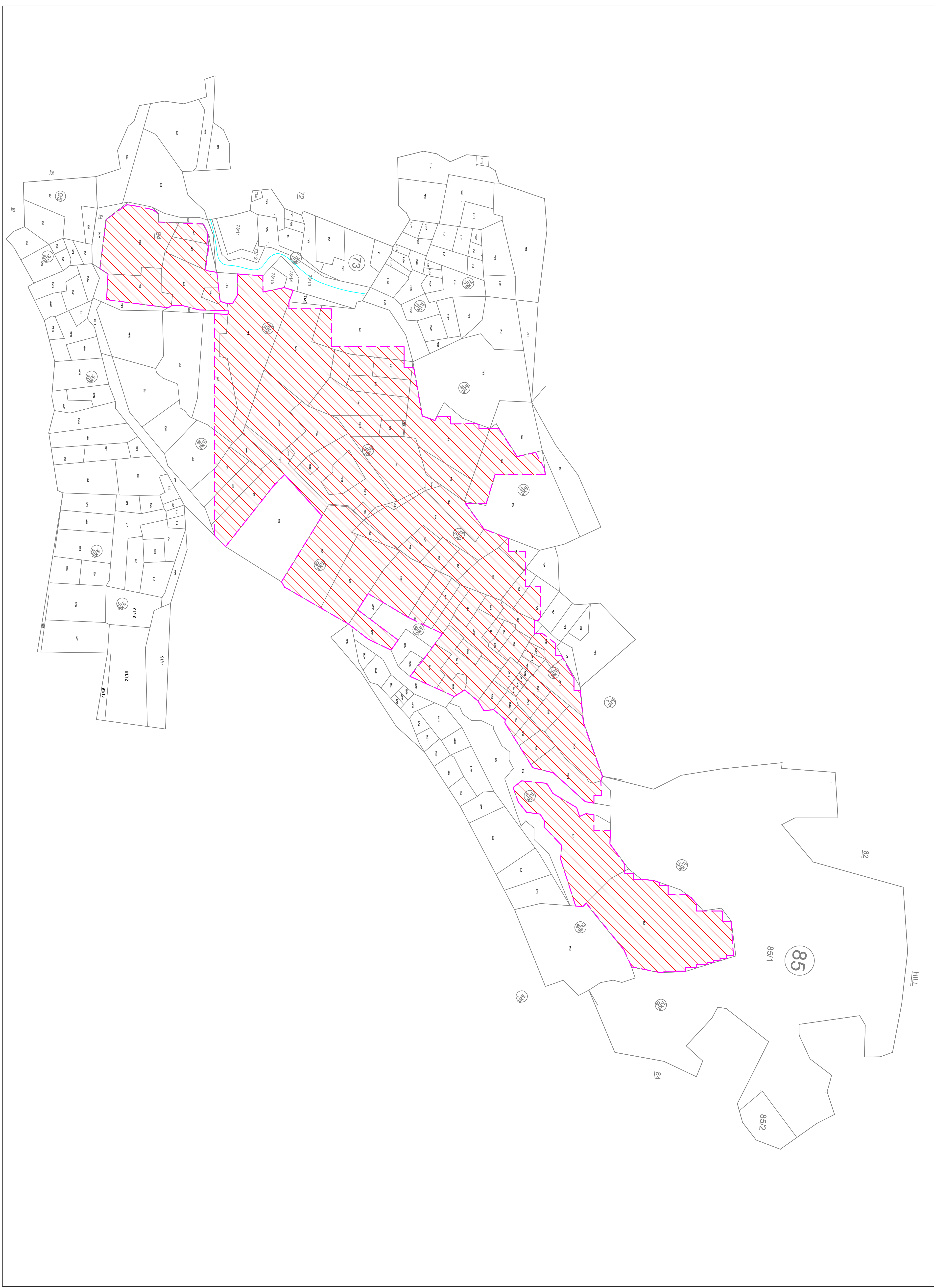
COMBINED SKETCH SHOWING THE PROPOSED LAYOUT IN S.Y. Nos. 74/p, 75/p, 76/p, 77/p, 78/p, 79/p, 86/p, 87/p, 88/p, 89/p, 90/p & 94/p OF RELI VILLAGE, KOTHAVALASA MANDAL, VIZIANAGARAM DISTRICT
