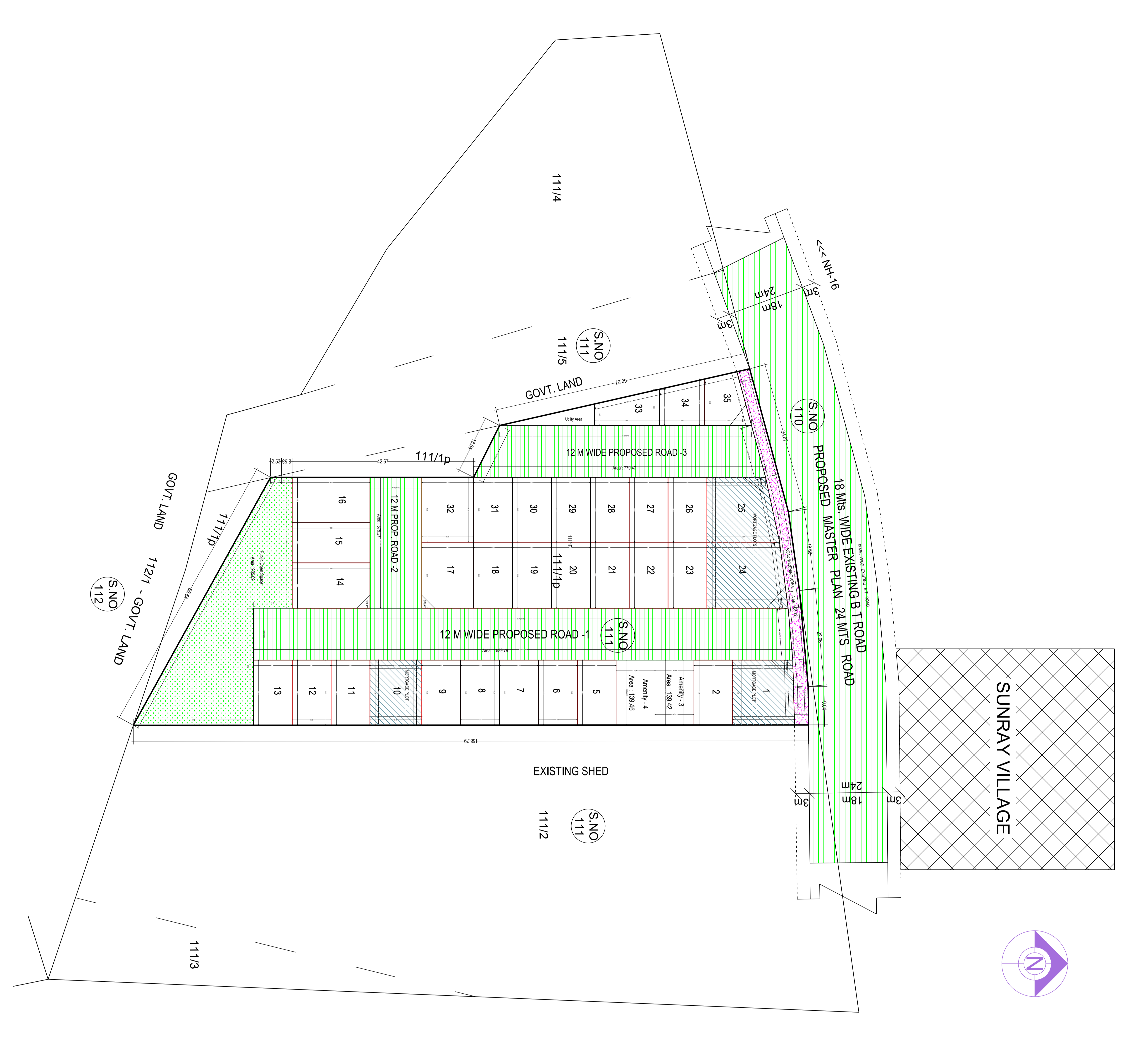
LAYOUT PLAN (Scale - 1:400)
