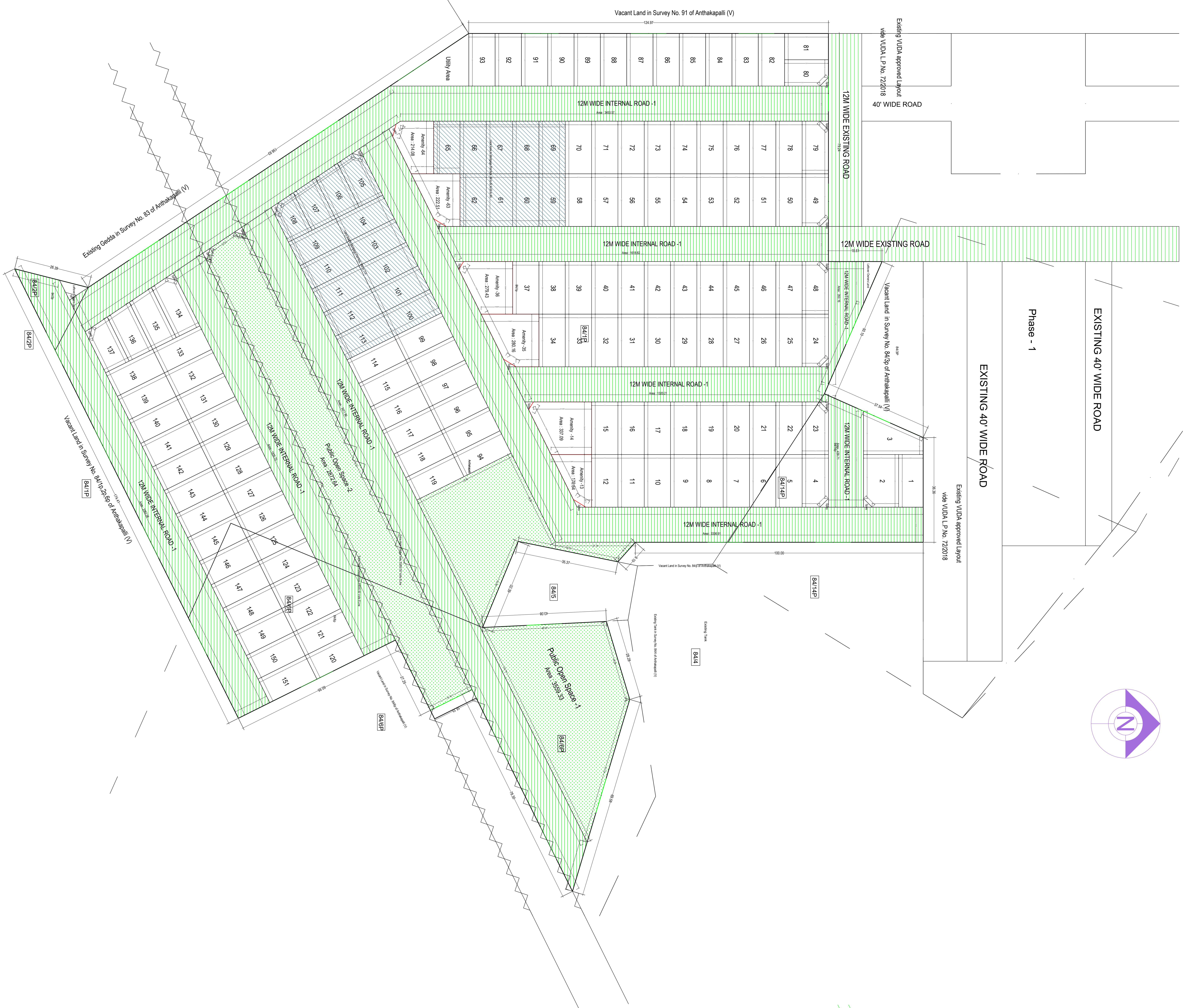
COMBINED PLAN SHOWING THE PROPOSED LAY OUT IN S. Nos. 84/1p, 2p, 3p, 4p OF ANTHAKAPALL VILLAGE, SABBAYRAM MANDAL, VISAKHAPATNAM DISTRICT NORTH
