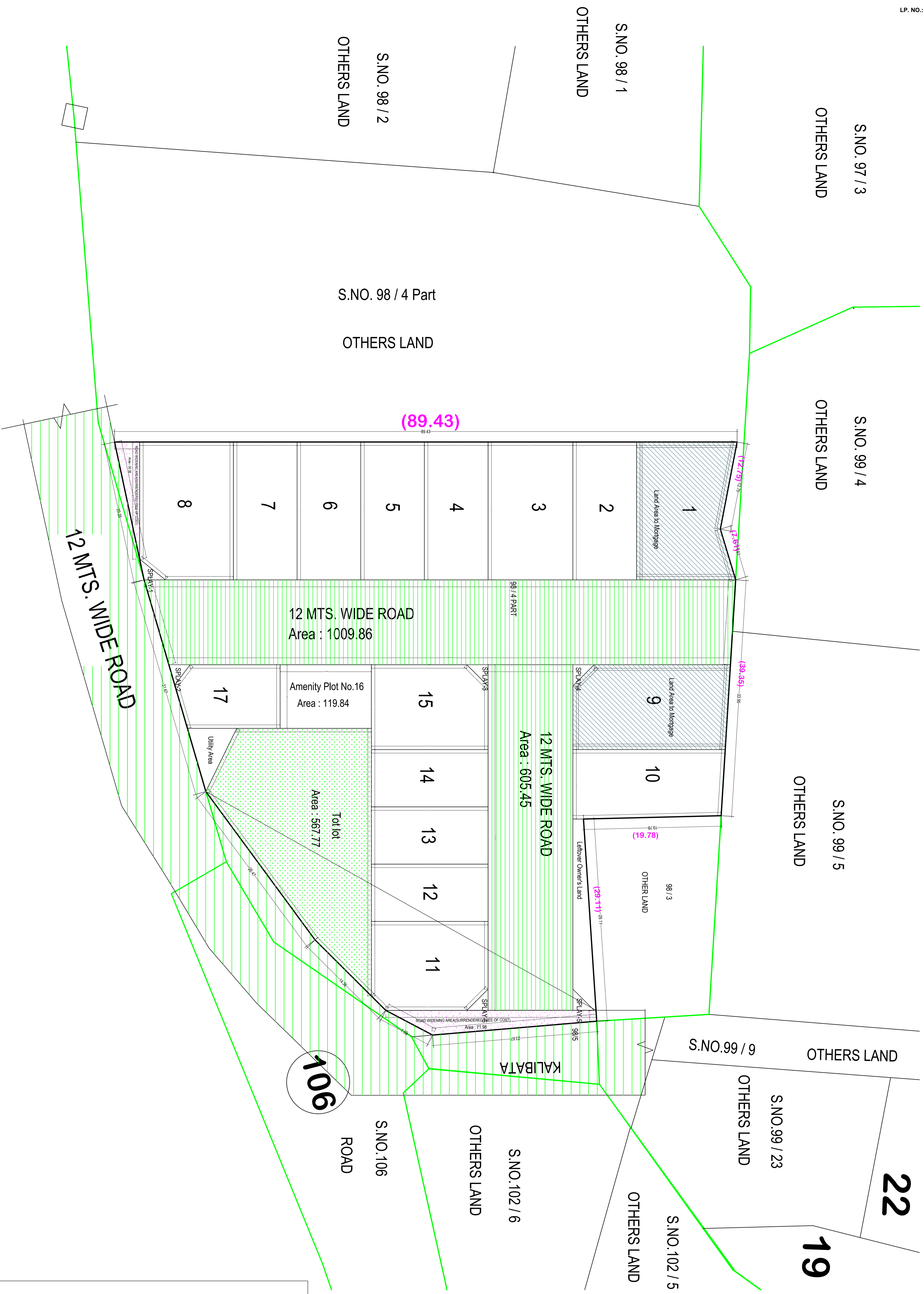
LAYOUT PLAN (Scale - 1:400)
