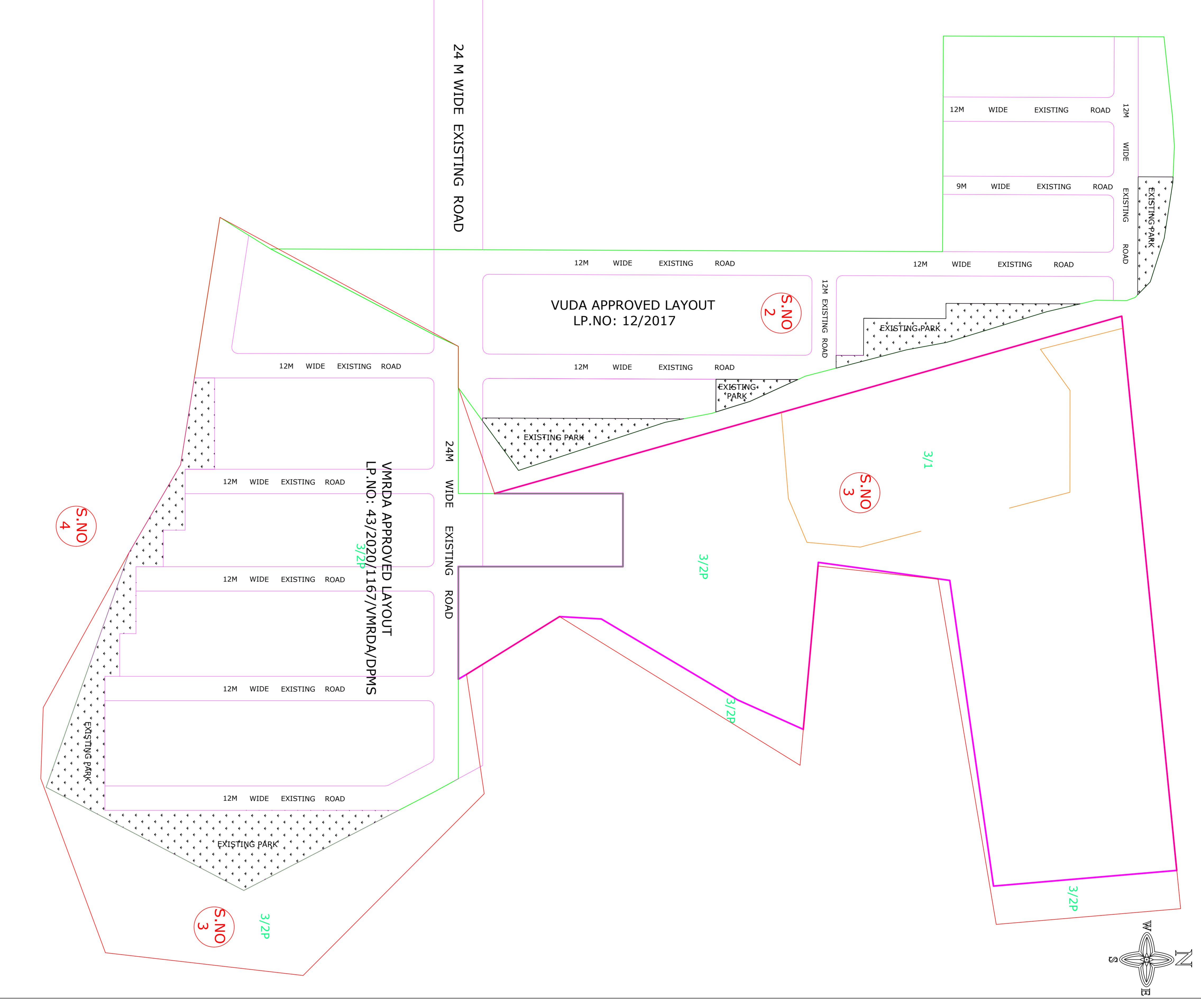
COMBINED FMB SKETCH IN S.No: 3/1 & 2p OF RELLU REVENUE VILLAGE, APPANNADHORAPALEM, KOTHAVALASA MANDAL, VIZIANAGARAM DISTRICT.
