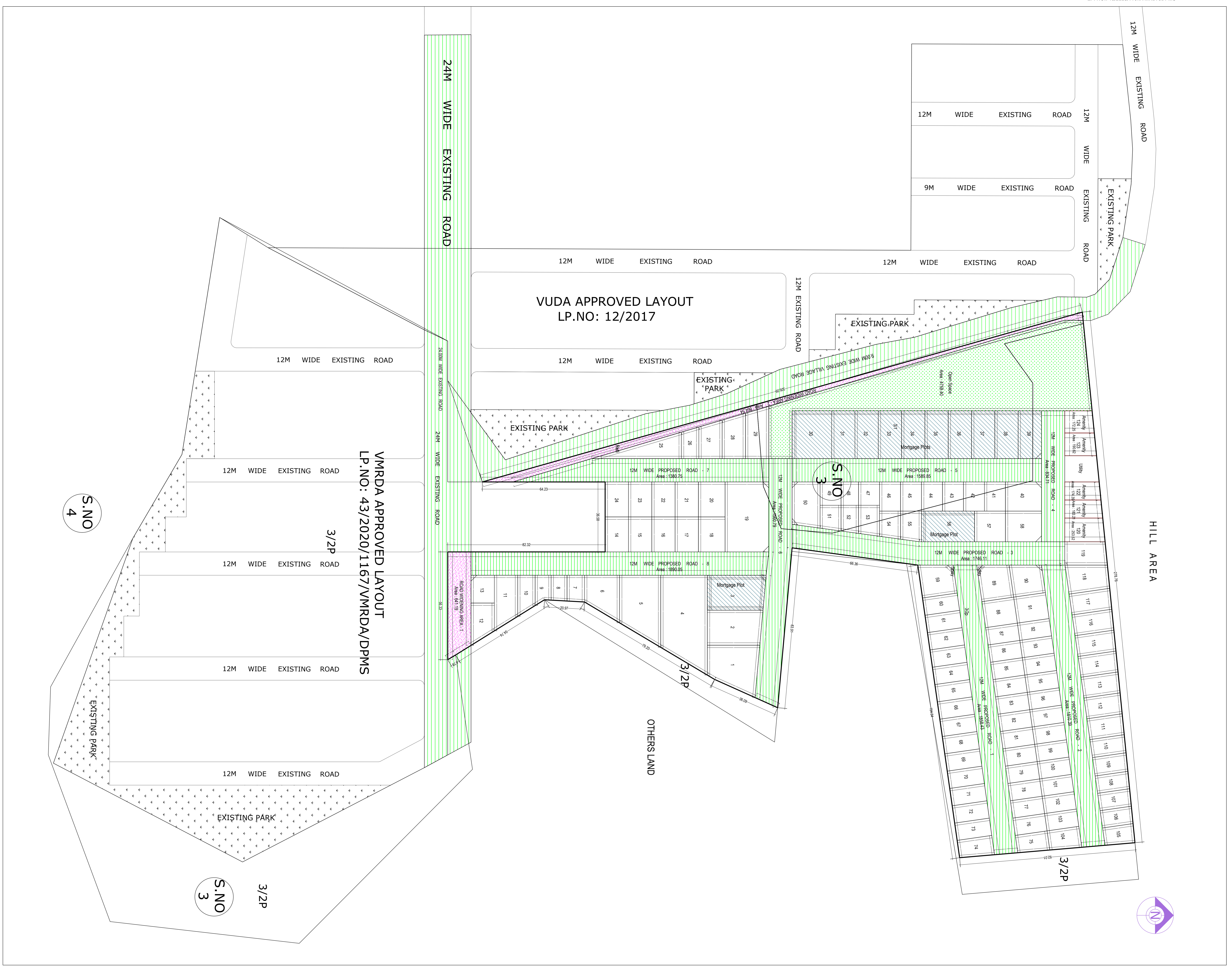
LAYOUT PLAN (Scale - 1:800)
