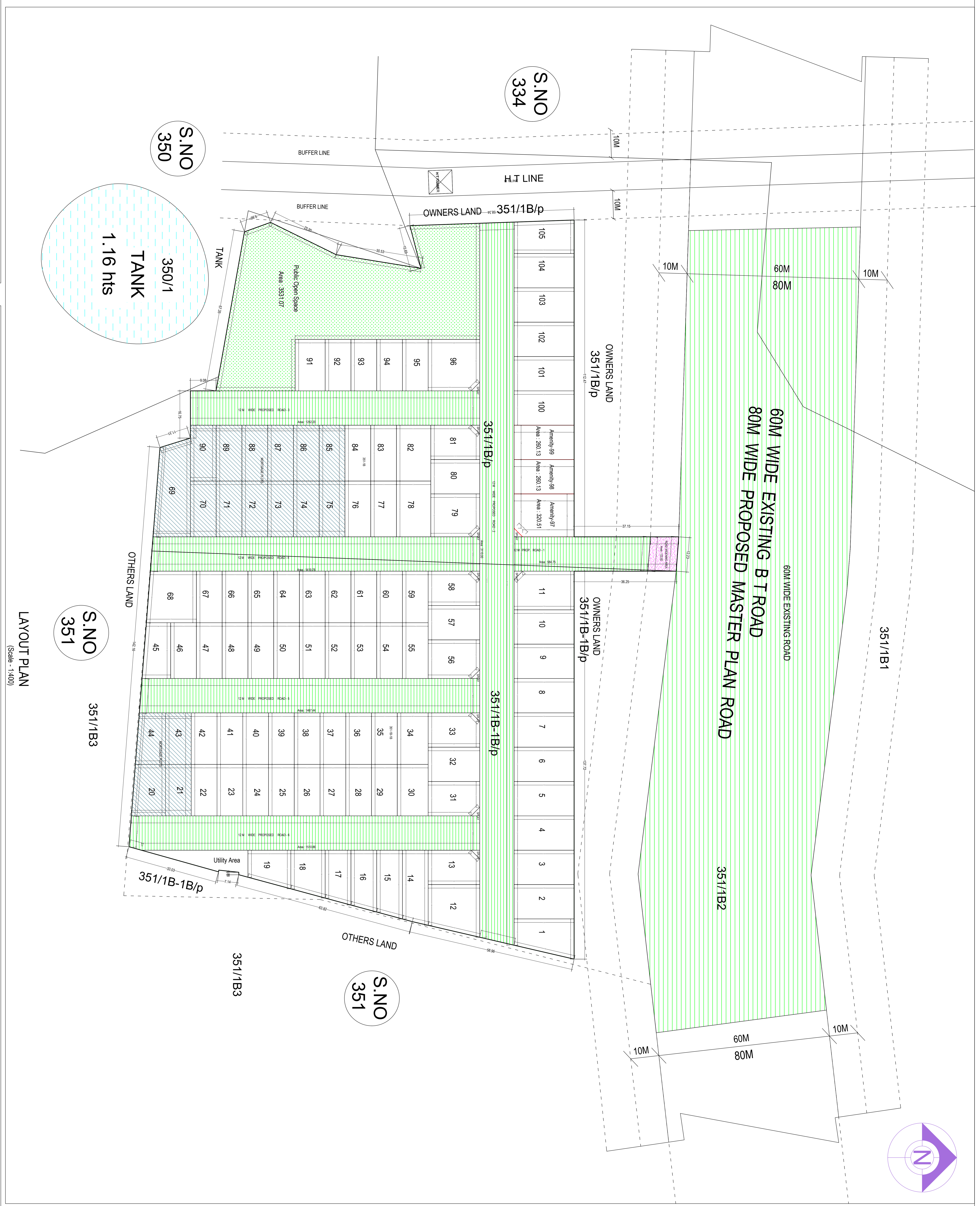
PMB SKETCH (N/S) NO.S/ 351/1B/p & 351/1B-1B/p OF SARIKA VILLAGE, VIZIANAGARAM MANDAL, VIZIANAGARAM DISTRICT.
