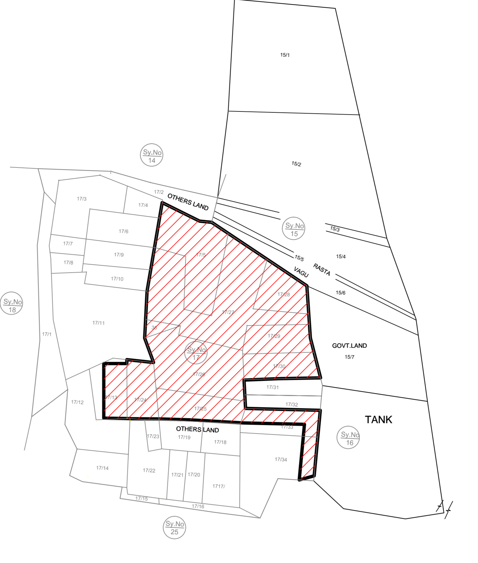
TOPO PLAN SHOWING THE PROPOSED LAYOUT SITE IN Sy.No.17/p OF ASKAPALLI VILLAGE, SABBAVARAM MANDAL, VISAKHAPATNAM DISTRICT
